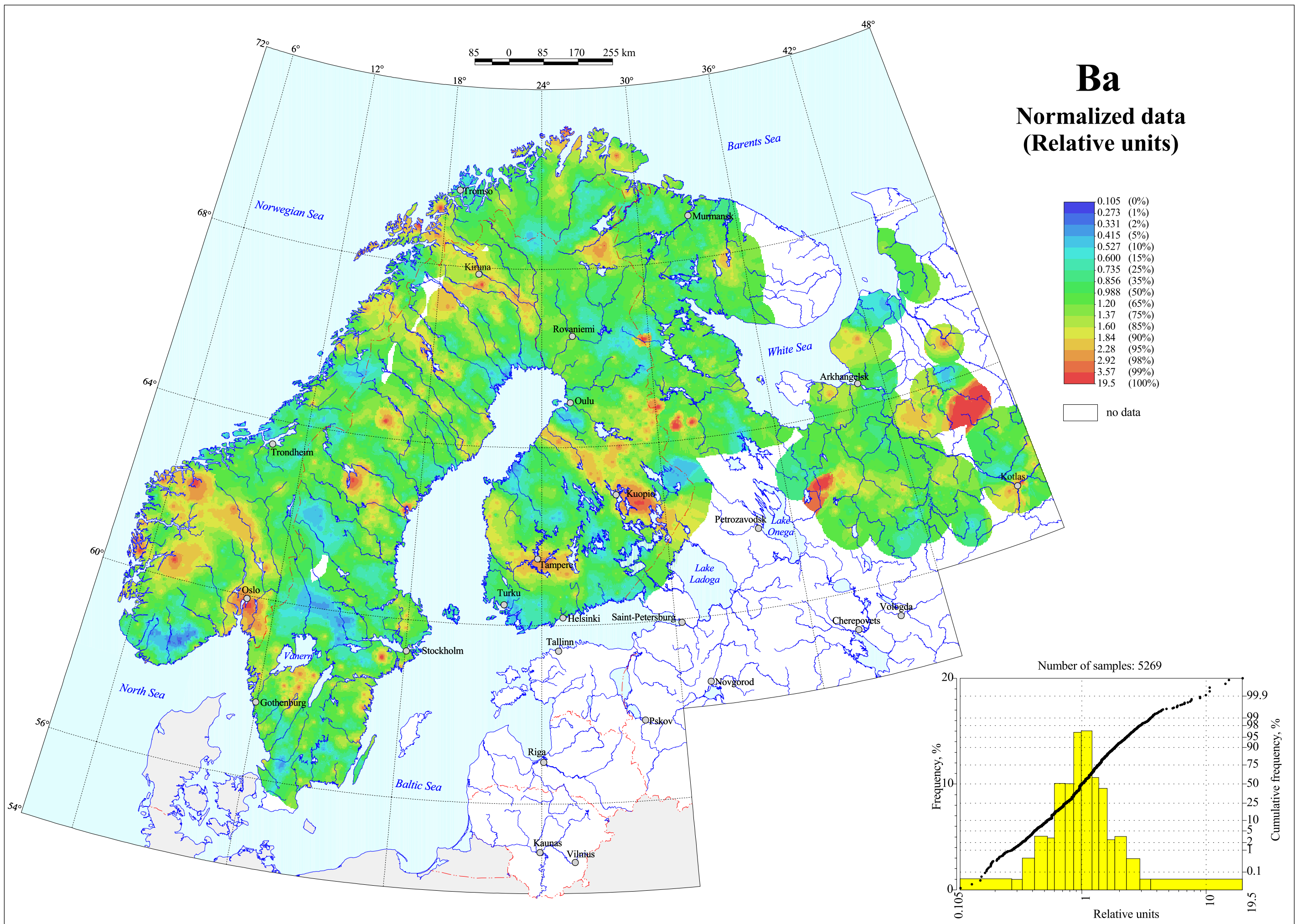
Barium in Till, Grain Size <0.06 mm
